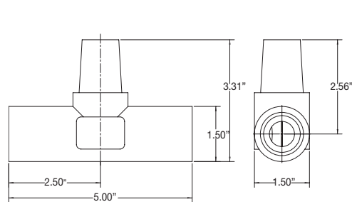
Three-Way Lay-Down "T" Connectors
