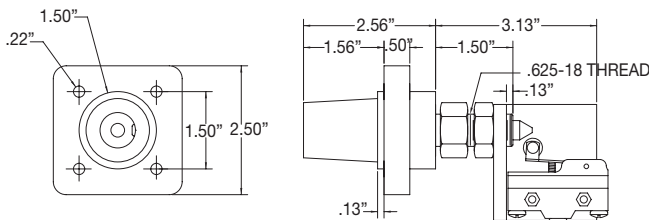
Female Receptacle Assembly With Interlock Switch
