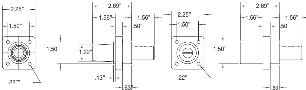
Female & Male E1016 Double Set Screw Receptacles
