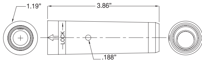
Male &amp; Female Plug
