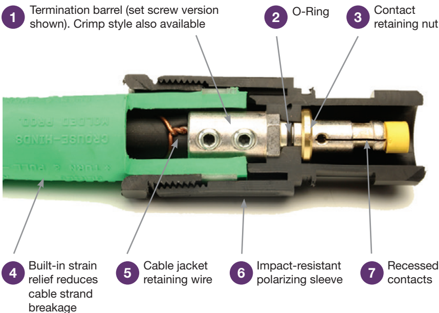
Cut-Away View of E0200 Male Plug
