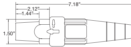
Female Non-Vulcanized Plug
