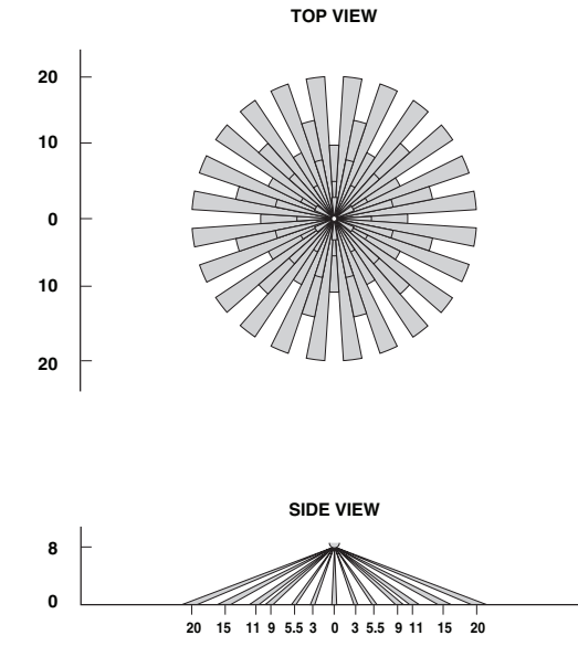
Figure 6 - (Cat. No. O3C15) - Field-of-View Ranges Extended range lens (black frame), mounting height (8-12 ft)
