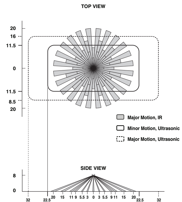
Figure 5 (Cat. No. O3C20) Field-of-View Ranges Extended range lens (black frame), mounting height (8-12 ft)
