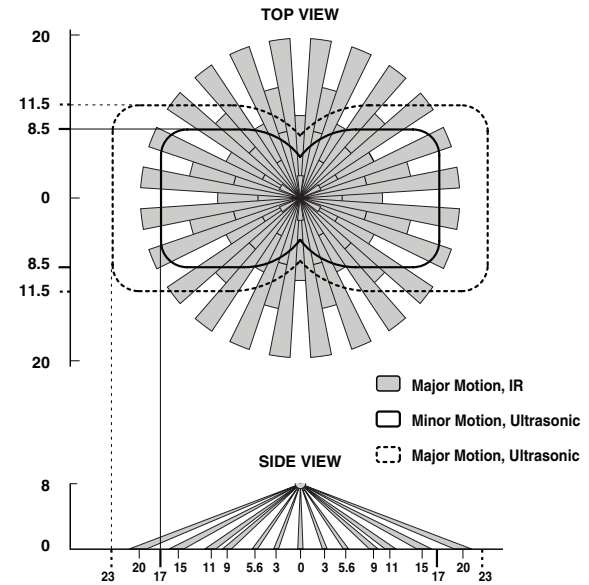
Figure 4 (Cat. No. O3C10) Field-of-View Ranges Extended range lens (black frame), mounting height (8-12 ft)
