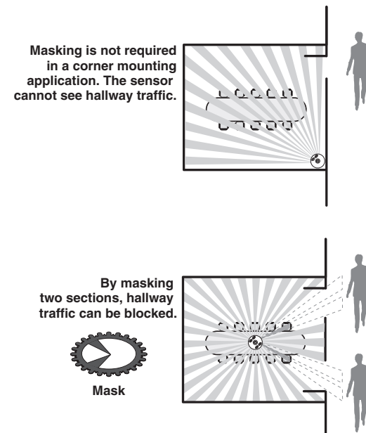
Figure 9 - Mounting Location Diagram
