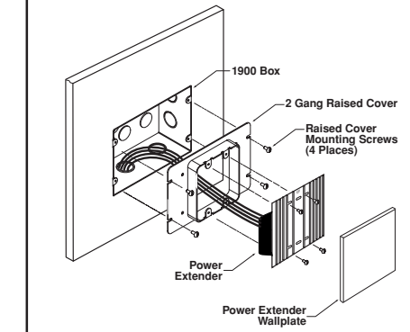
Figure 1B: Flush Mounting
