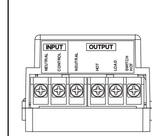
Figure 2: End View
