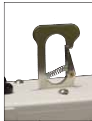
Spring-lock hook allows contractors to mount the unit in seconds, without the need for tools.
