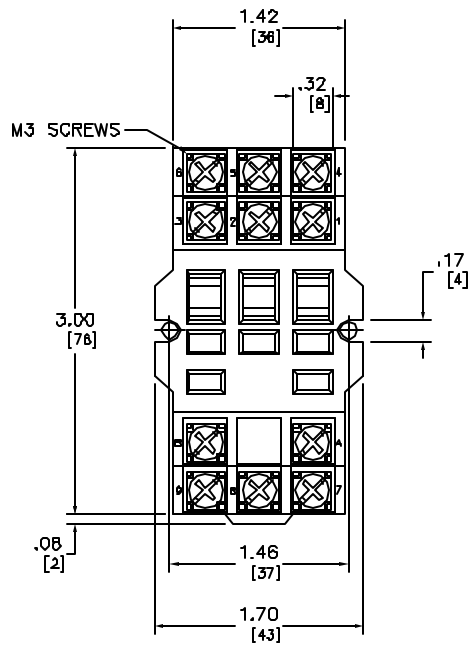
FRONT VIEW SHOWN WITHOUT RELAY INSTALLED
