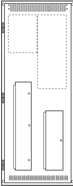
Figure 17: 36 in. w x 91.5 in. x 24 in. d Type 1 Enclosure
