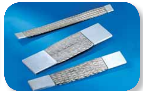
ERIFLEX® Braids
